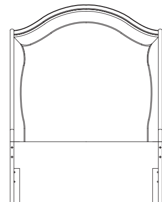
012-930 PANEL HEADBOARD 3/3 - TWIN W42 D4 H49 (107 x 10 x 124cm) Bored for frame. pages: 2/3, 14
