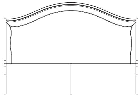
012-901 DAYBED BACK PANEL W75 D3 H52 (191 x 8 x 132cm) pages: 12/13, 14
